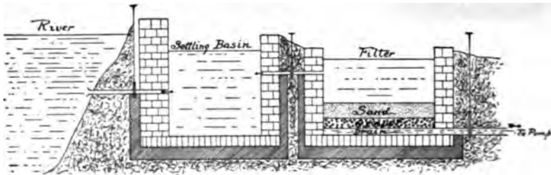
Fig. 168.—Cross-section of filter plant (after Hazen).
